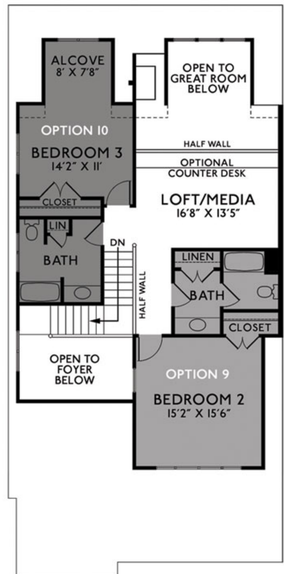
Optional Second Floor with 2 Bedrooms, 2 Baths, & Loft/Media Room
