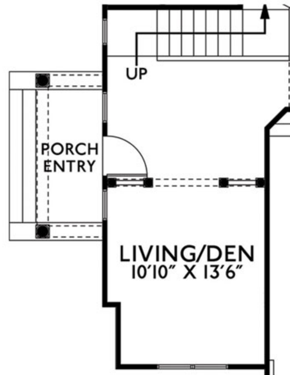
Optional Porch Entry with Columns and Roof
