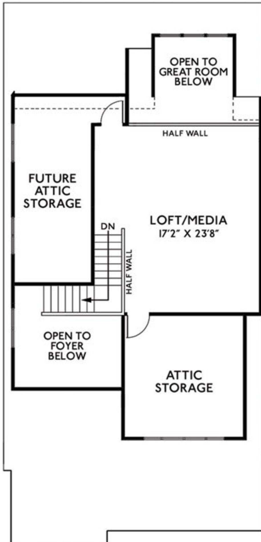
Optional Second Floor Plan with Loft/Media Room
